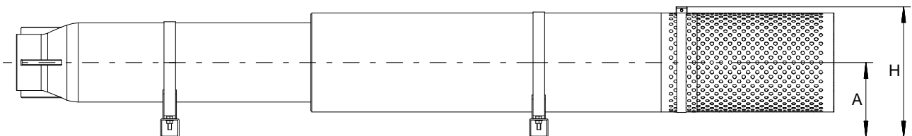
Pic. 2: Suction jacket, horizontal
