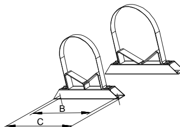
Pic. 3: supporting brackets
